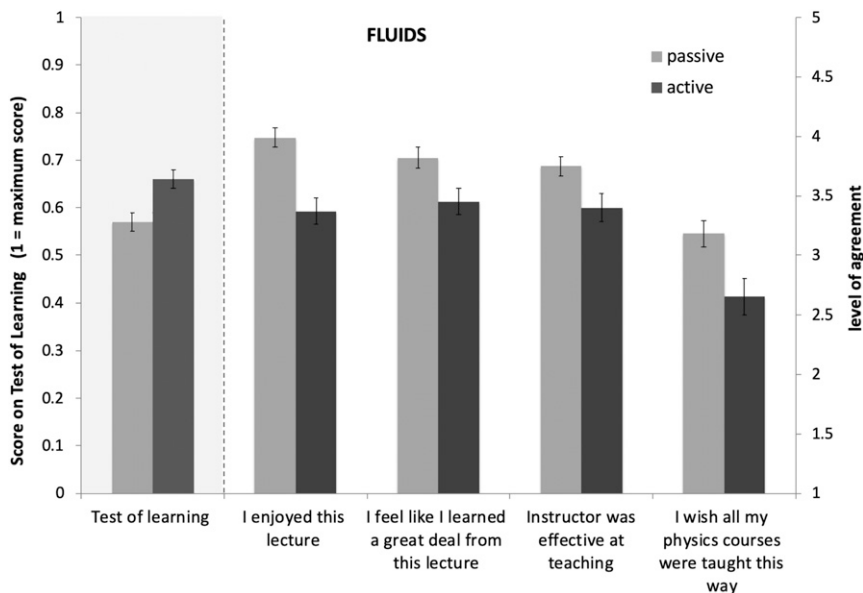
Fig. 2. A comparison of performance on the TOL and FOL responses between students taught with a traditional lecture (passive) and students taught actively for the fluids class. Error bars show 1 SE.
